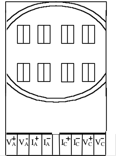
Form 5S (SWRGS5) wiring diagram
